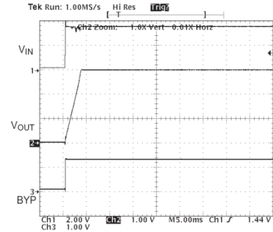
Fig. 17: Fast V_{IN} = 1000 \mu F Output Load
