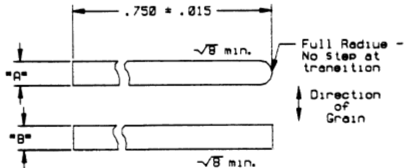
Dimensions - Inch
