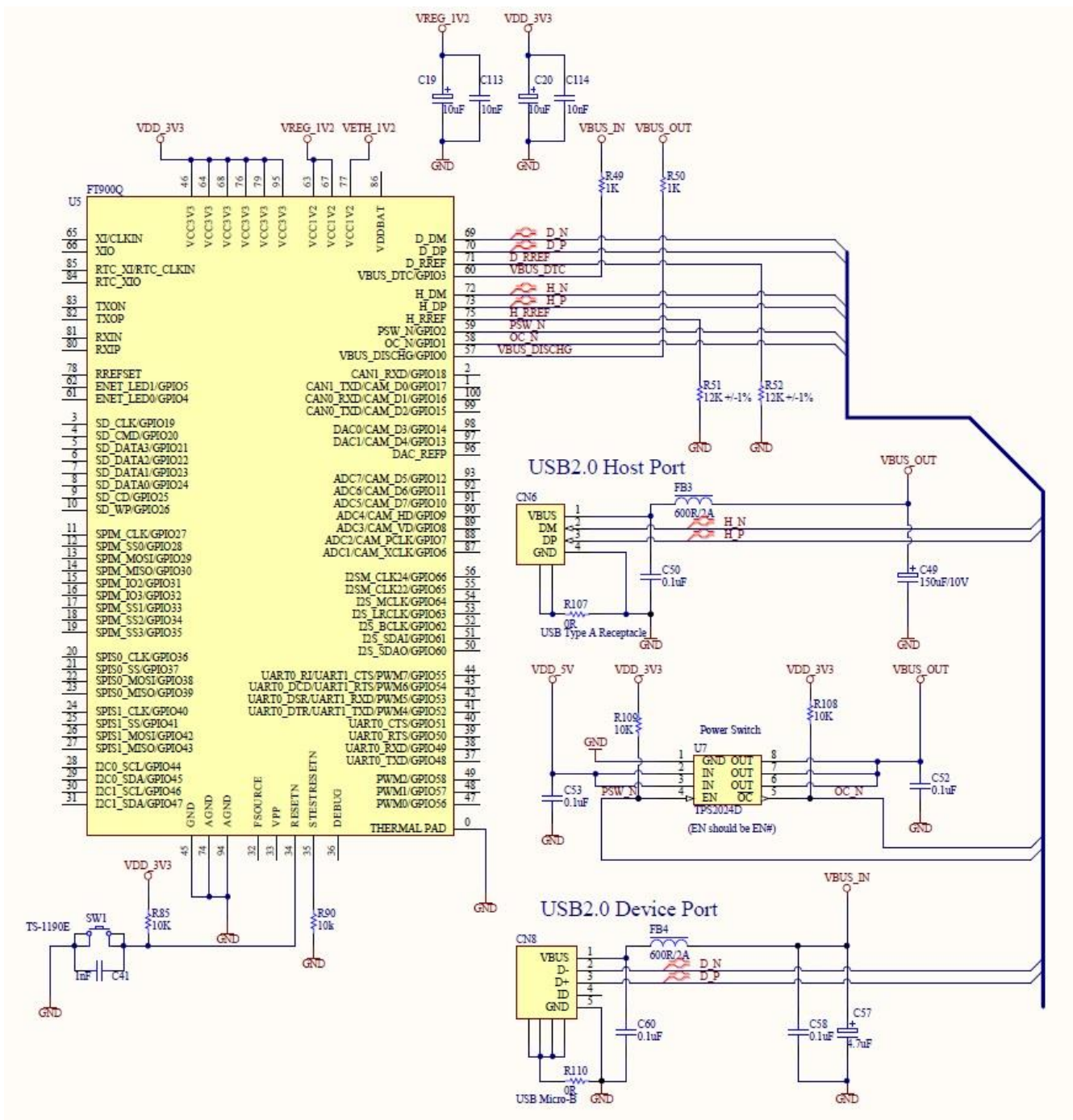
Figure 4-6 – USB Connectors
