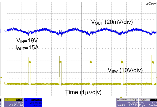
Figure 21. Static Load Ripple at Full Load
