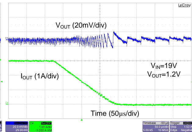
Figure 23. Operation as Load Changes from 3 A to 0 A
