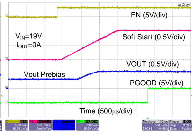
Figure 19. Startup Waveforms with Pre-Bias Voltage on Output
