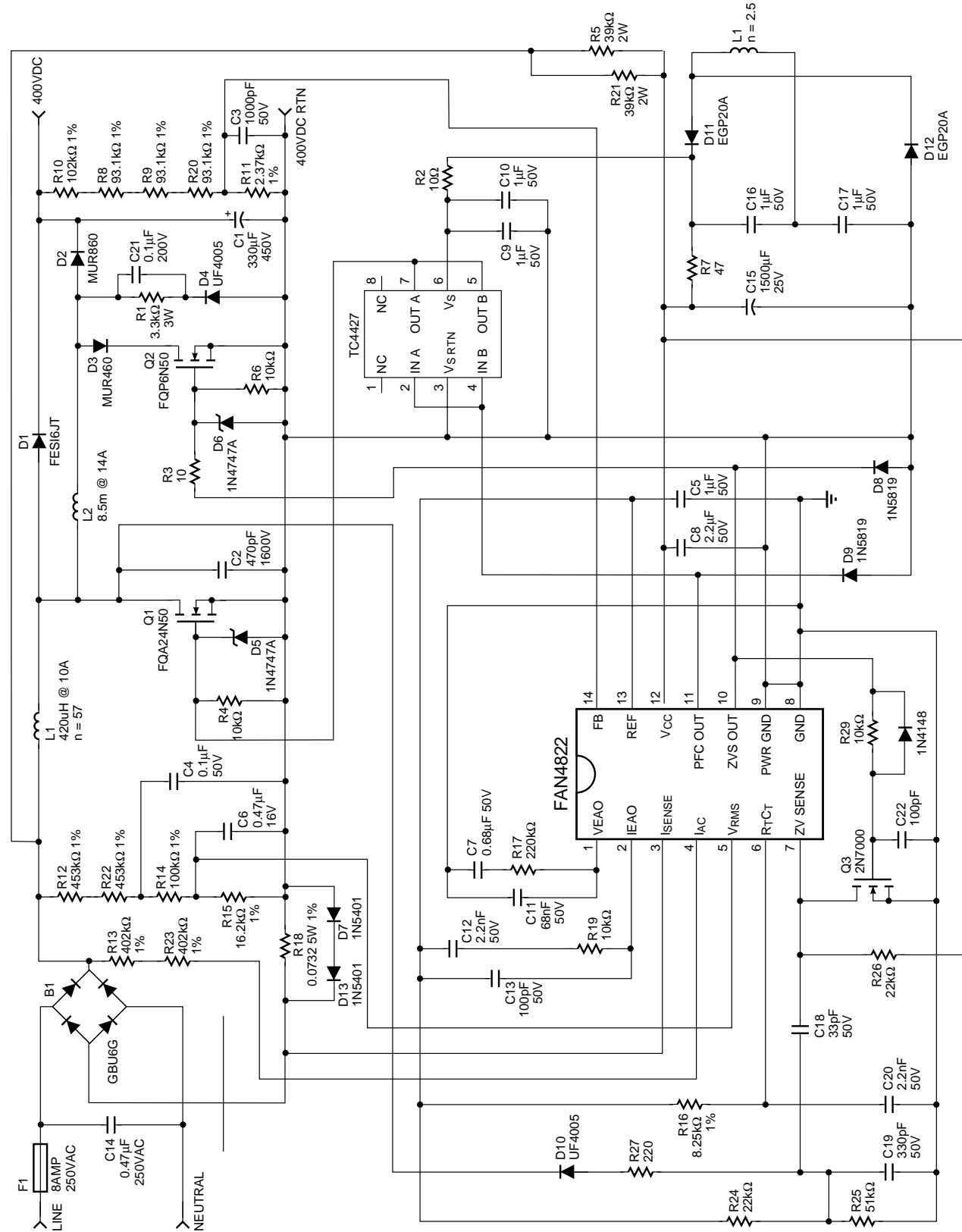
Figure 3. FAN4822 Schematic.
