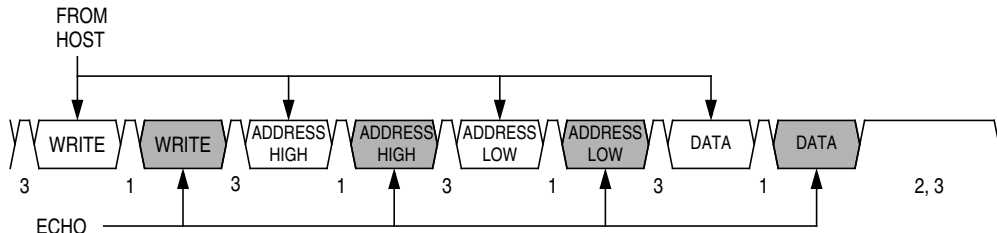
Figure 18-14. Read Transaction
