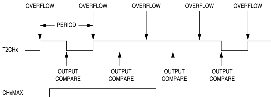
Figure 17-11. CHxMAX Latency
