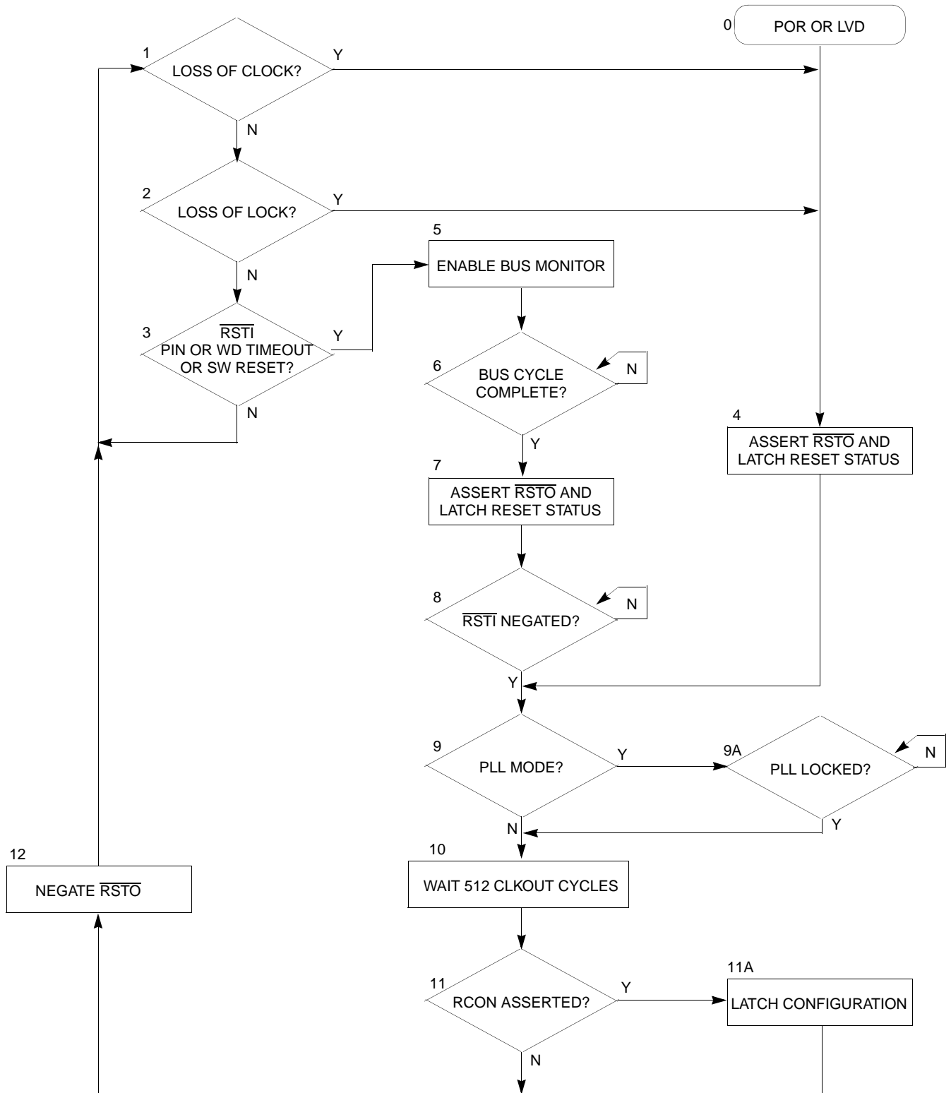
Figure 29-4. Reset Control Flow
