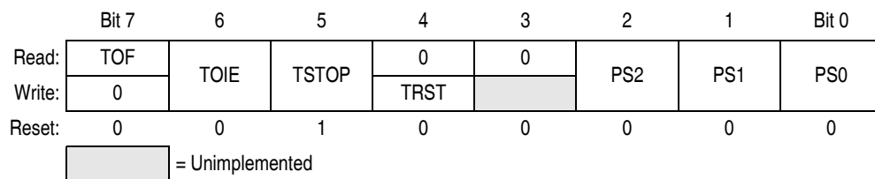
Figure 14-4. TIM Status and Control Register (TSC)
