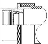
STYLE 2 (STRAIGHT - See Note 1)
