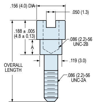
Figure 1 #2-56 Jackpost
