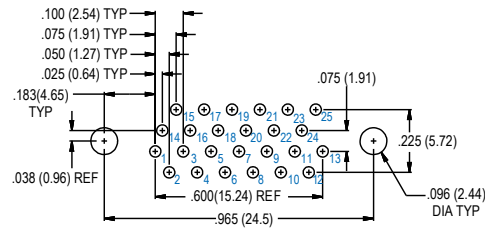
25 SOCKET
