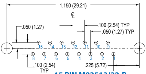
15 PIN M83513/22-B
