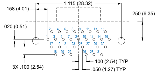
31 PIN
