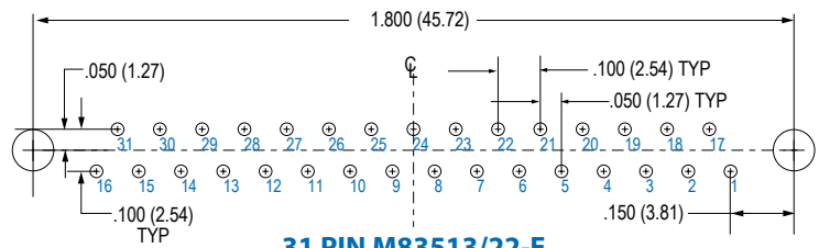
31 PIN M83513/22-E
