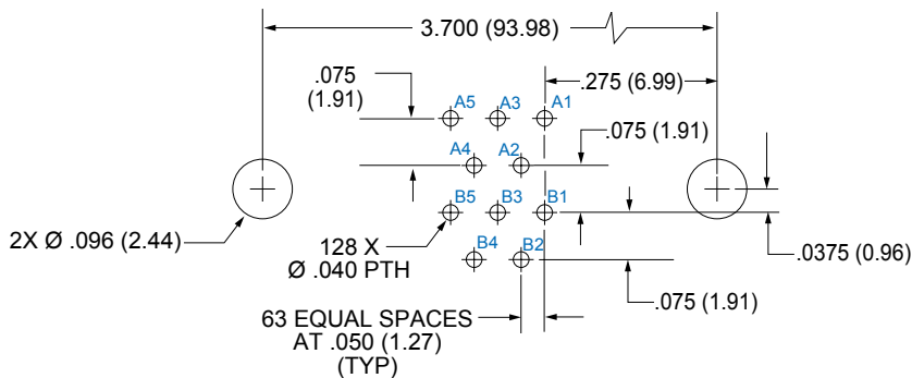
PATTERN SHOWN IS FOR CONNECTOR MOUNTING SIDE OF PC BOARD
