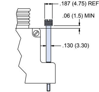
Typical Jackscrew
