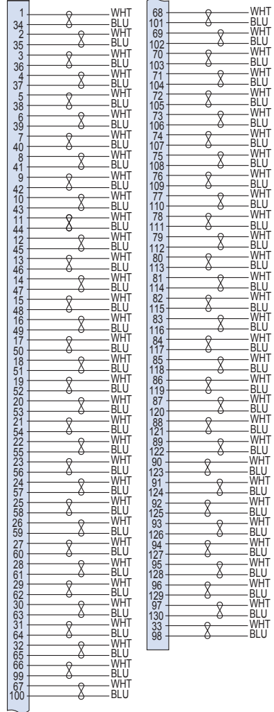
130 Contacts
