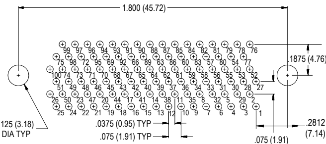
100 PIN M83513/30-H
