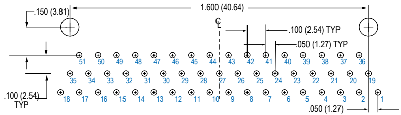
51 PIN
