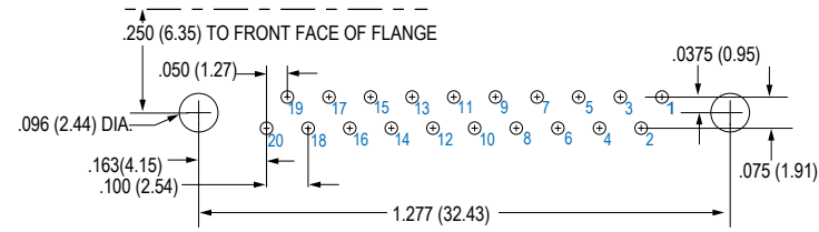
20 PIN
