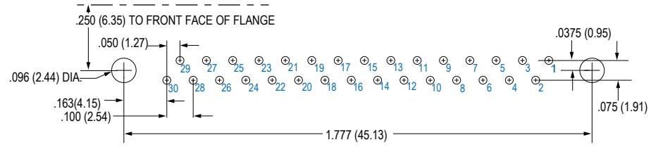
30 PIN
