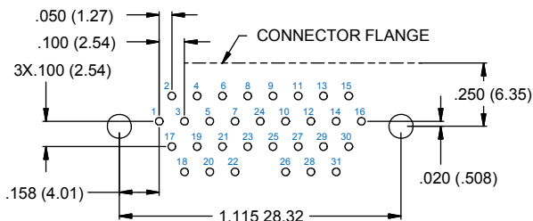
31 PIN
