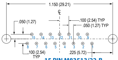
15 PIN M83513/22-B
