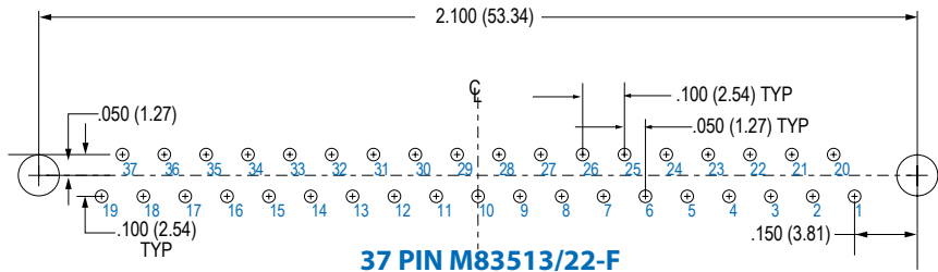
37 PIN M83513/22-F
