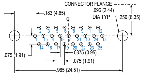
25 PIN
