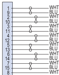
15 Contacts
