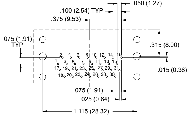
31 PIN
