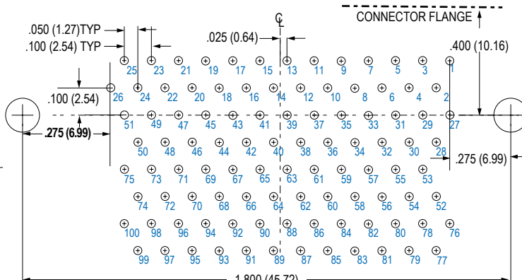
100 SOCKET M83513/15-H
