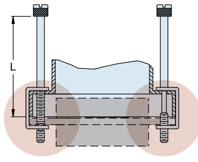
Code EJ Extended Jackscrew Code E Floating Extended Jackscrew
