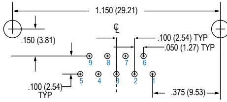
9 PIN
