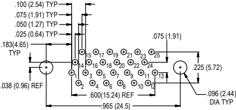
25 SOCKET
