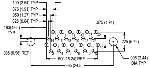
25 SOCKET
