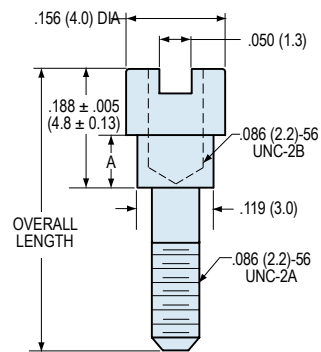
Figure 1 #2-56 Jackpost
