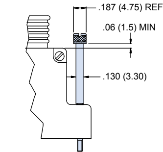
Typical Jackscrew
