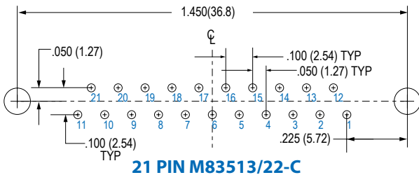
21 PIN M83513/22-C
