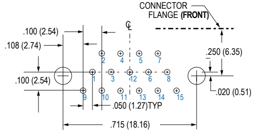
15 PIN M83513/10-B
