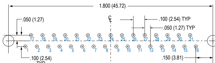
31 SOCKET M83513/25-E
