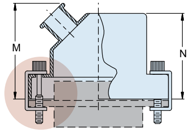
Code H Extended Jackscrew
