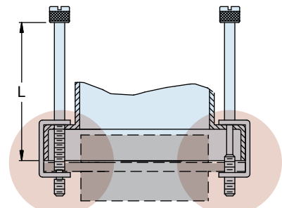
Code EJ Extended Jackscrew Code E Floating Extended Jackscrew
