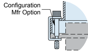
Code HJ Hex Socket Jackscrew
