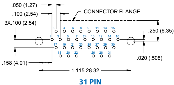
31 PIN
