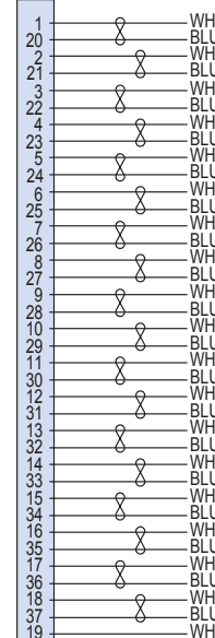
37 Contacts
