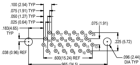
25 SOCKET
