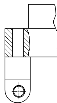
Board Mount Threaded Insert
