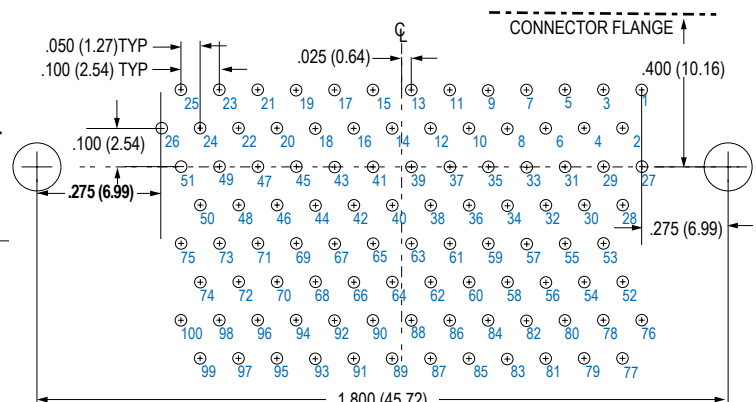
100 SOCKET M83513/15-H
