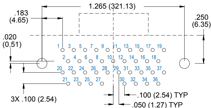
37 PIN
