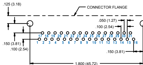
31 SOCKET M83513/19-E
