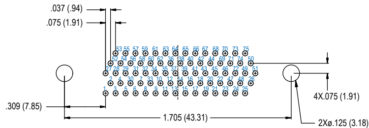
75 SOCKET
