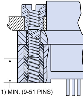
RU Style Rear Panel Jackpost with Threaded Insert
