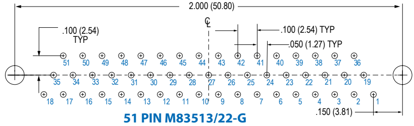
51 PIN M83513/22-G
