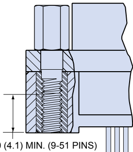
PU Style Jackpost with Threaded Insert
