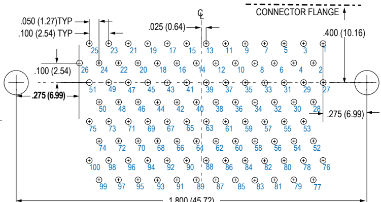
100 SOCKET M83513/15-H
