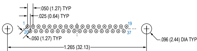
37 CONTACTS
