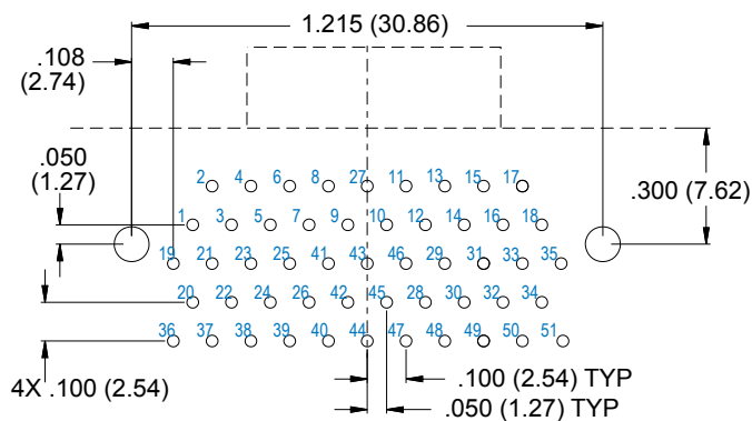
51 PIN
