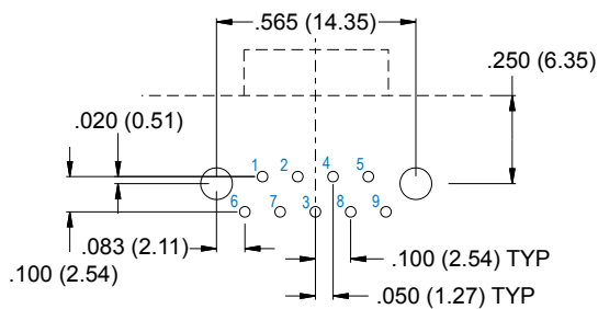
9 PIN
