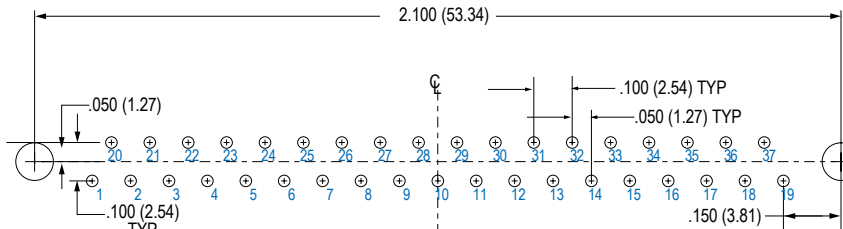
37 SOCKET M83513/25-F
