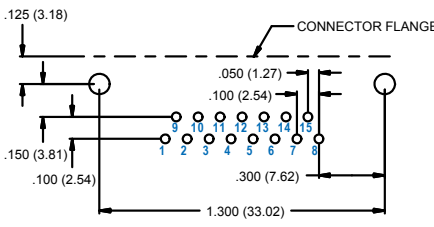
15 SOCKET M83513/19-B
