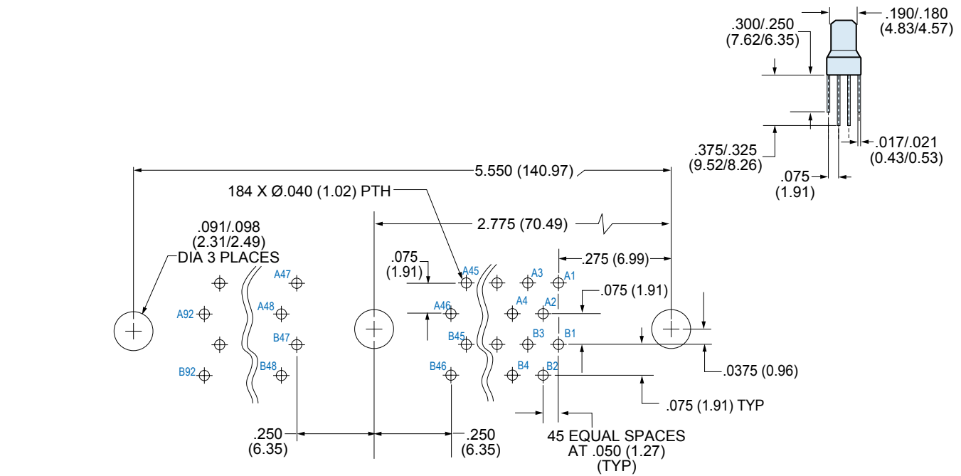
PATTERN SHOWN IS FOR CONNECTOR MOUNTING SIDE OF PC BOARD
